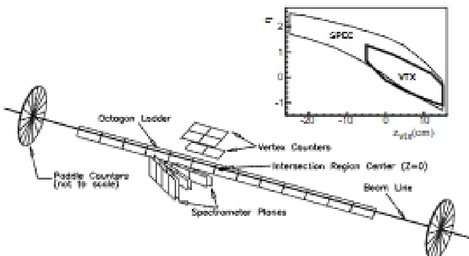
FIG. 1. Detector setup for the initial running period. The insert shows the \eta acceptance of the SPEC and VTX subdetectors as a function of primary vertex position.
