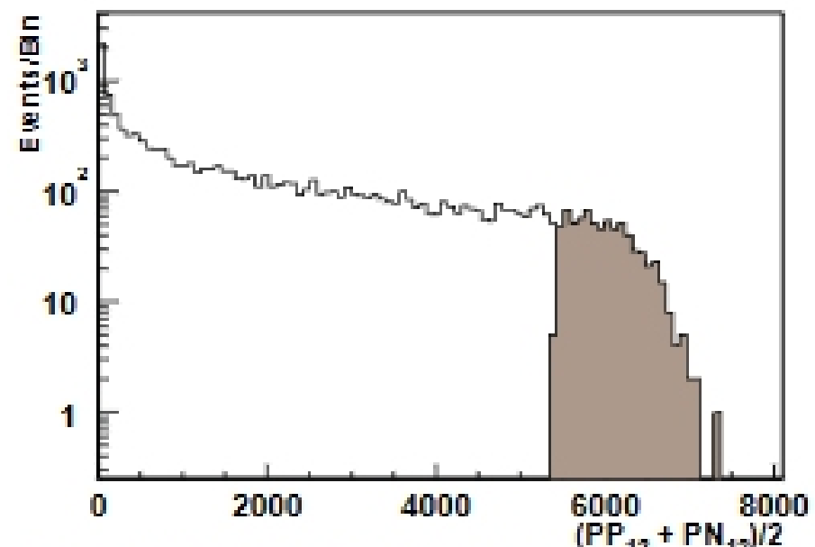
FIG. 2. Paddle signal distribution for data events at \sqrt{s} = 130 AGeV.
