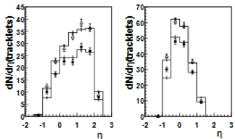
FIG. 3. Tracklet pseudorapidity density in the detector acceptance per event for data at \sqrt{s} = 56 (circles) and 130 AGeV (triangles) for SPEC (left) and VTX (right), in comparison to scaled HIJING simulations (solid lines).
