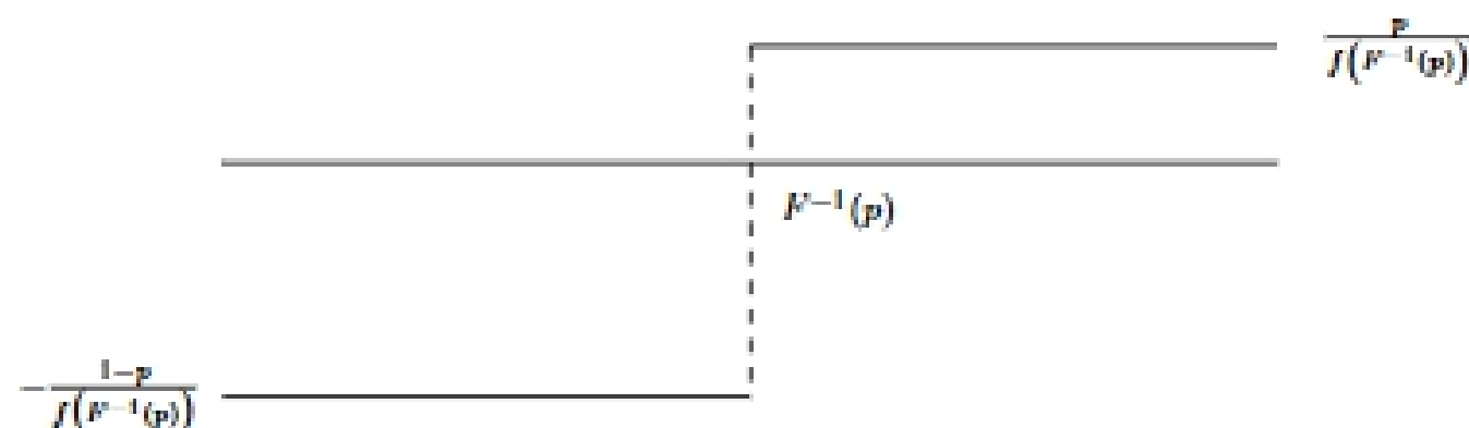
Figure 1: Influence function of the p th quantile
