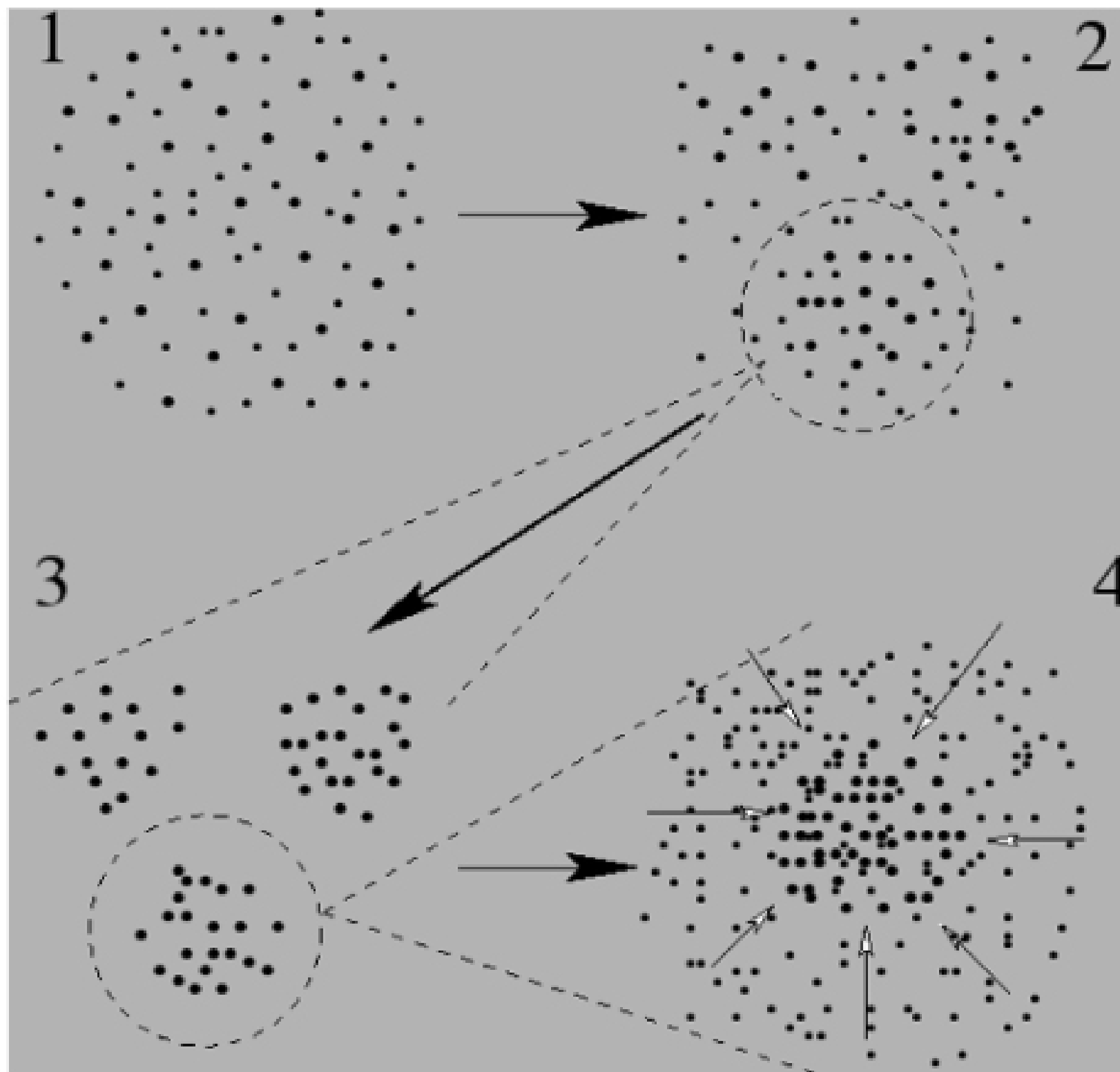
Fragmentation of molecular cloud
