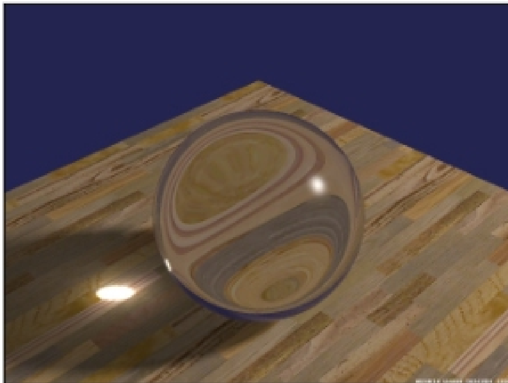
Caustic Sphere Henrik Jensen (refraction caustic)
