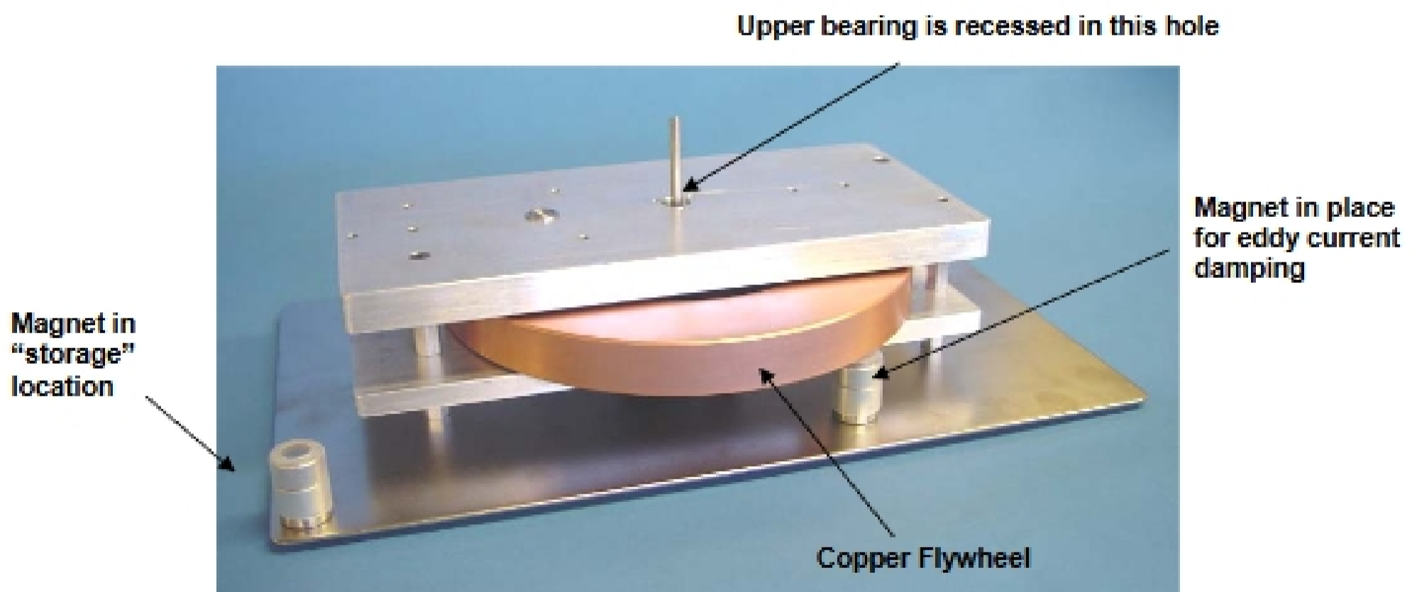
Figure 1. The copper flywheel and bearings.
