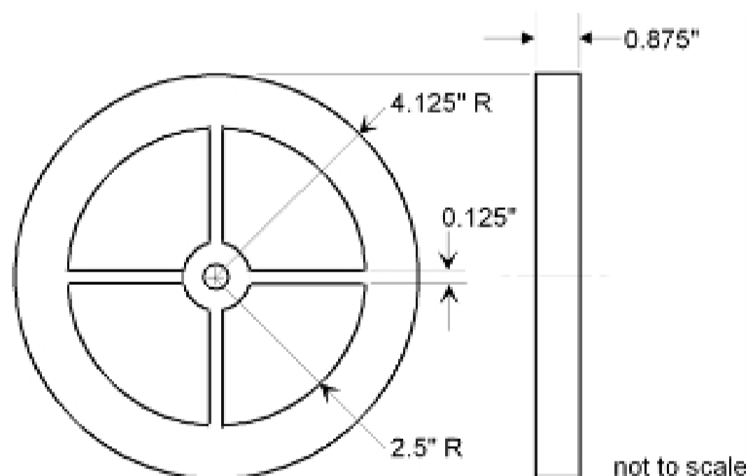
Figure 3. Dimensions of the copper flywheel.
