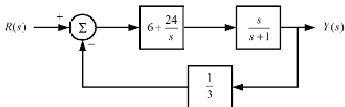
Figure 1: Block diagram of a feedback control system.
