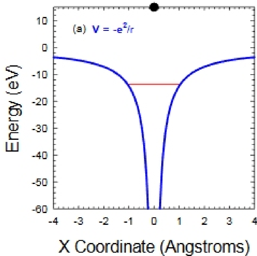
H atom
