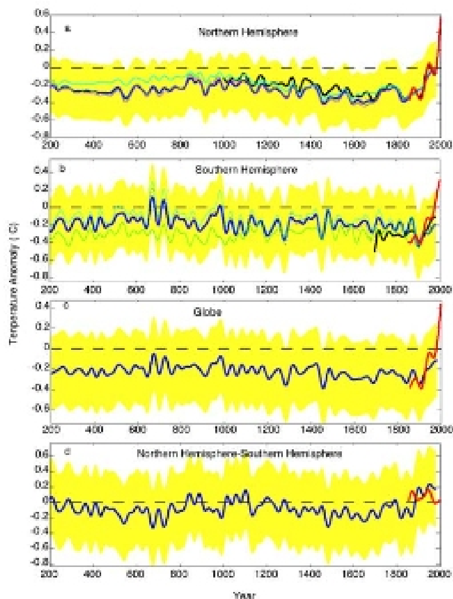
Figure 2. Hemispheric temperature reconstructions ('standard reconstructions' based on area and local correlation weighting, shown as thick blue). All series are anomalies based on 1961–1990 instrumental reference period (mean shown by dashed line), and smoothed with a 40 year lowpass filter. Smoothed instrumental series are shown by thick red curve (the constraint employed by the filter preserves the late 20th century trend). 95% confidence intervals for the standard reconstructions are shown by yellow shading. (a) NH reconstruction based on 6 indicators available back to AD 200. Also shown are NH reconstructions based on areal and hemispheric correlation weighting (green), areal weighting only (magenta), local-correlation weighting only (cyan) [blue dotted curve shows standard reconstruction based on all 8 indicators available back to AD 553]. Shown for comparison is millennial composite of previous shorter reconstructions discussed in text (thick black). (b) SH reconstruction based on 2 indicators back to AD 200 (thick blue) and 3 indicators back to AD 470 (blue dotted). Other weighting schemes shown using color convention of (a). Shown for comparison is multi-century composite of previous reconstructions discussed in text (thick black). (c) global mean (average of NH and SH) surface temperature reconstruction, and (d) interhemispheric temperature contrast (Northern minus Southern Hemisphere mean).
