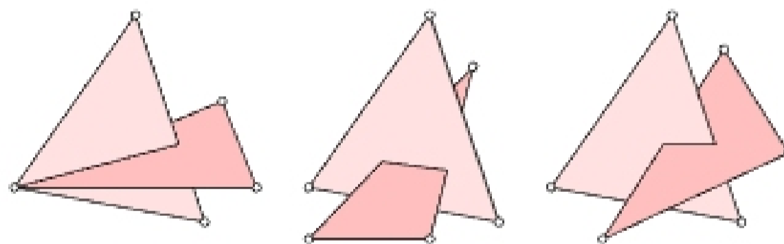
Figure II.11: The three ways two triangles in general position in \mathbb{R}^3 can cross each other.
