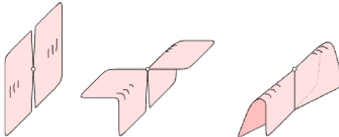
Figure II.10: Constructing the Whitney umbrella from a disk.
