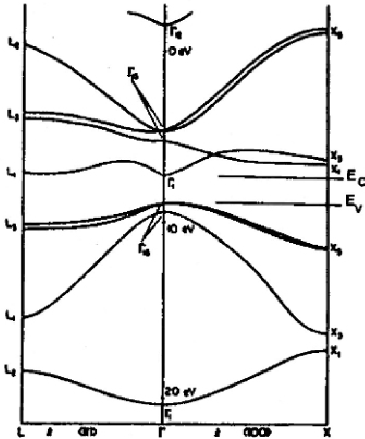
Band structure of GaAs in the (100) & (111) directions
