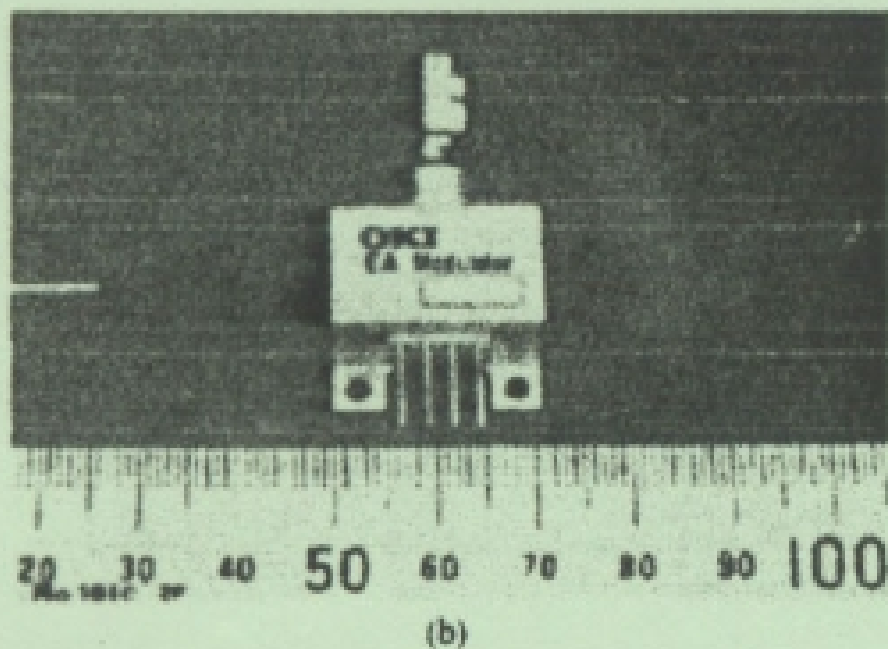
3. (a) Configuration and (b) photograph of EA modulator module.
