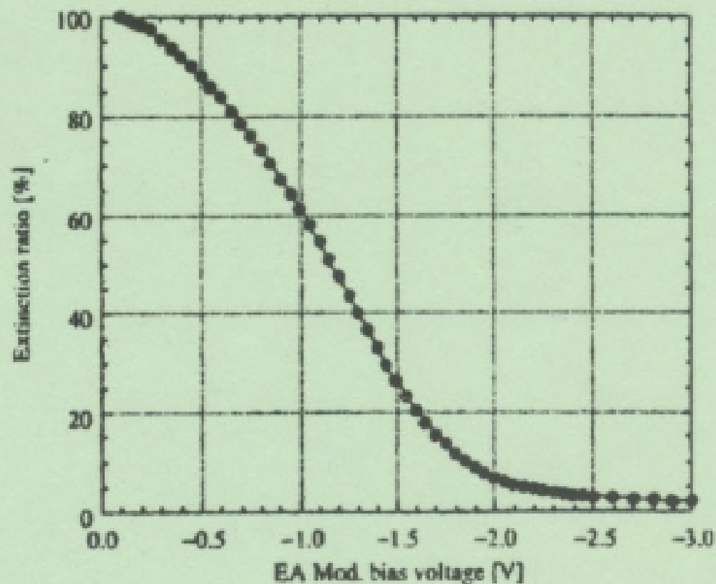
Fig. 5. Extinction ratio of EA modulator.
