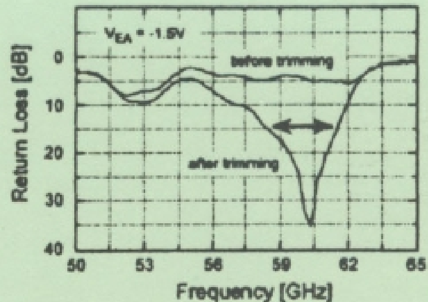
Fig. 4. Return loss of RF input power to the module.
