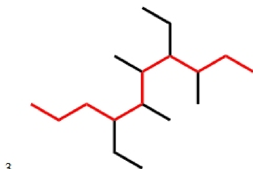
4,7-diethyl-3,5,6-trimethyldecane
