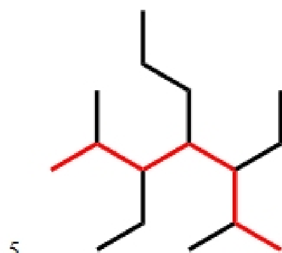
3,5-diethyl-2,6-dimethyl-4-propylheptane
