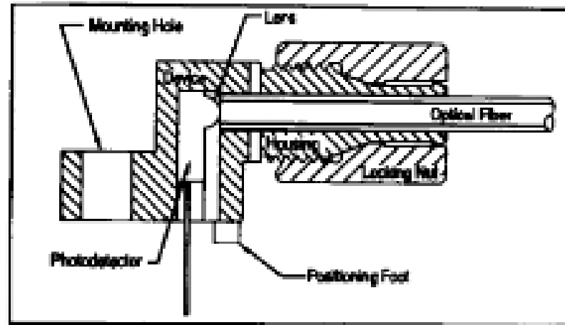
FIGURE 3. Cross-section of fiber optic device.
