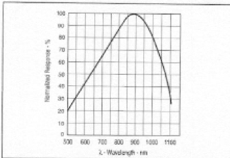
FIGURE 1. Typical detector response versus wavelength.
