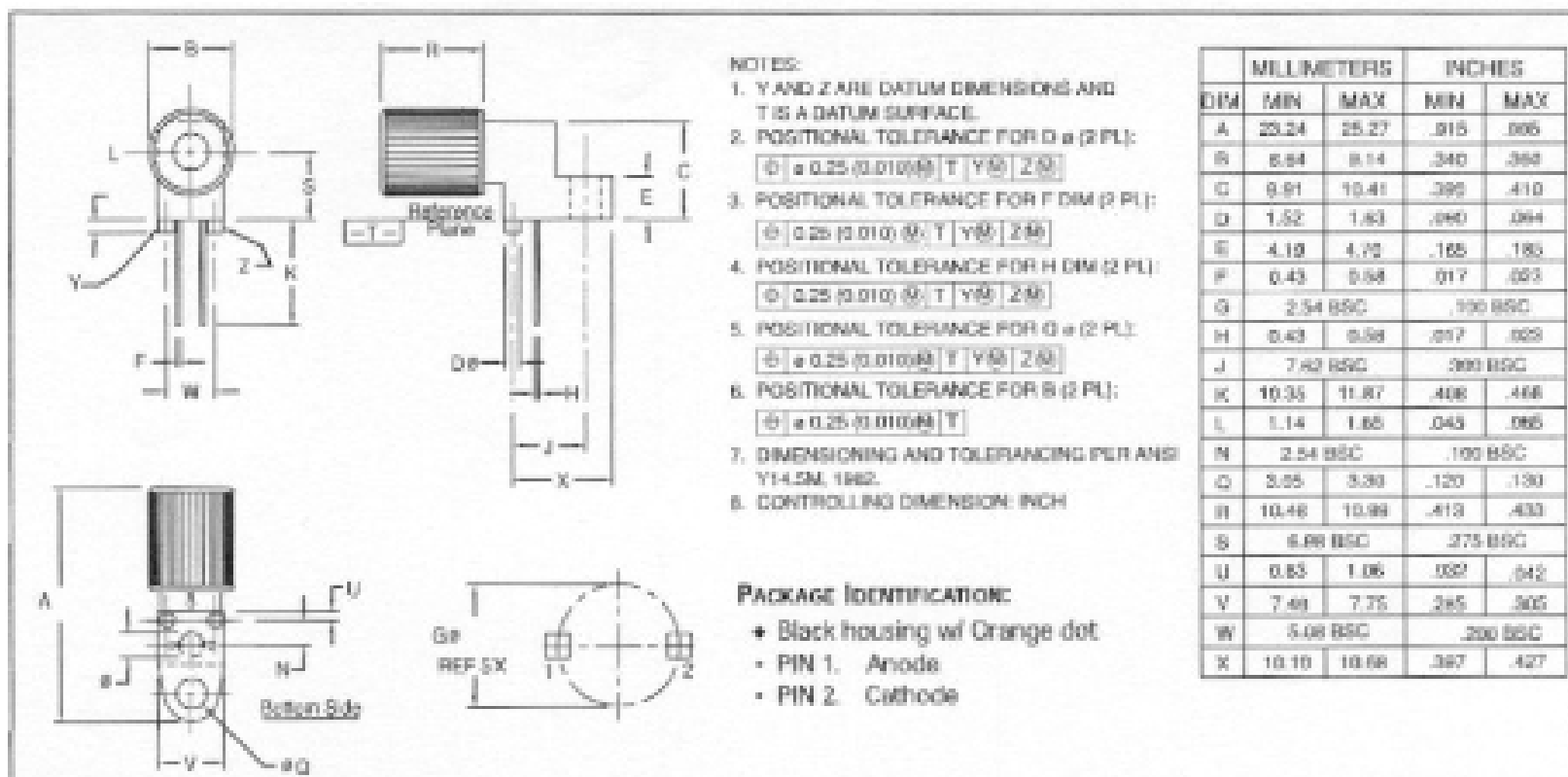
FIGURE 4. Case outline.
