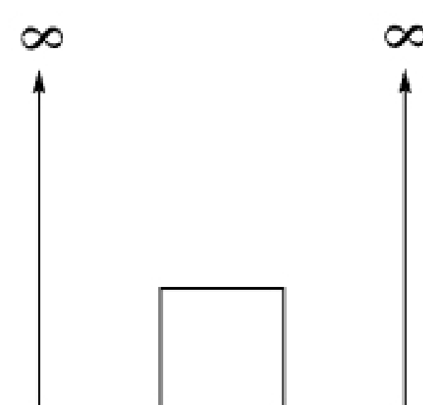
Particle in a double well
