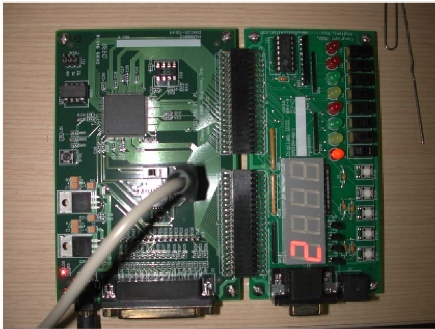
Figure 1: The D2XL and DI01 boards with programming cable attached.
