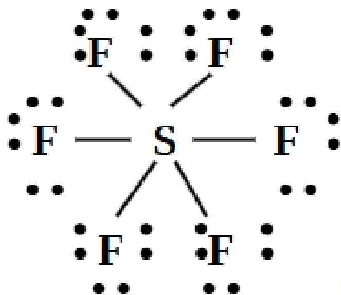
Sulfur hexafluoride
