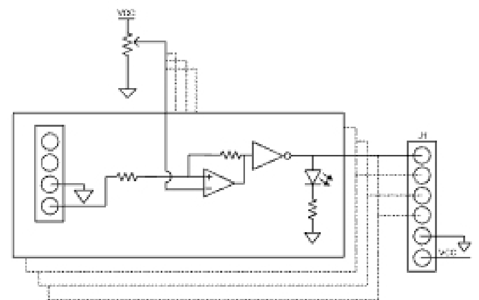
Figure 1 PmodLS1 Circuit Diagram
