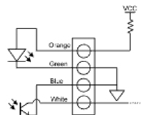
Figure 2 Sensor Connection Diagram
