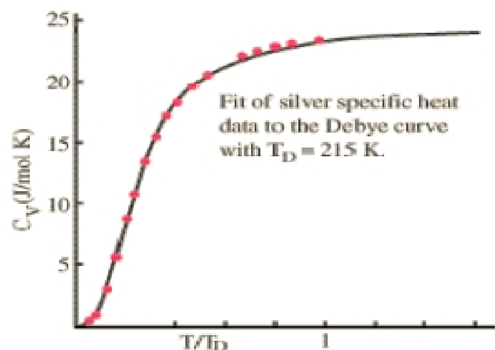
Fig. 2. Low Temperatures Specific Heat of Silver [5].
