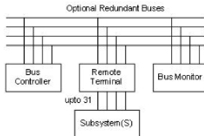
Figure 1. 1553 Multiplex Architecture
