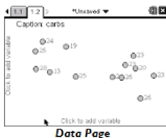
Choosing One Variable Stats
