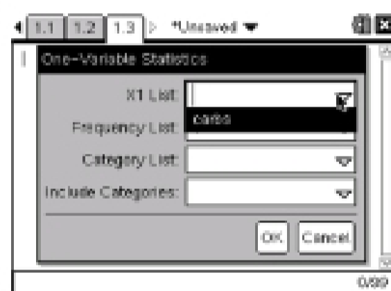
Choosing One Variable Stats
