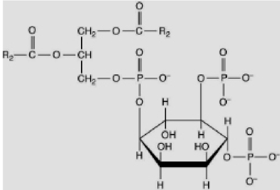
Phosphatidylinositol 4,5-bisphosphate (PIP 2 )
