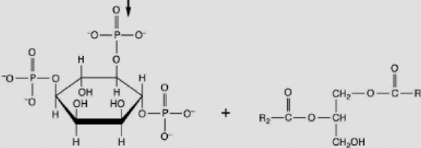
Inositol 1,4,5-trisphosphate (IP 3 ) + Diacylglycerol (DAG)
