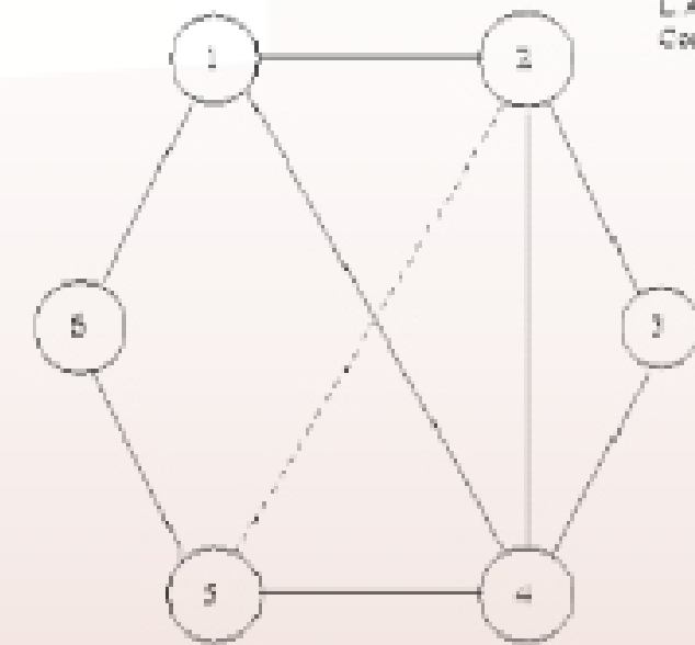
Undirected Graph
