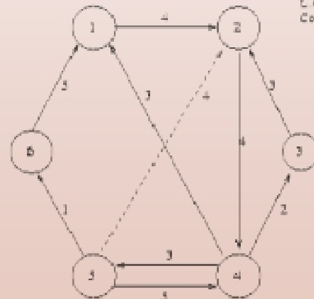
Weighted Directed Graph
