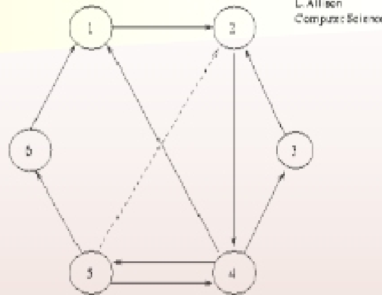
Directed Graph
