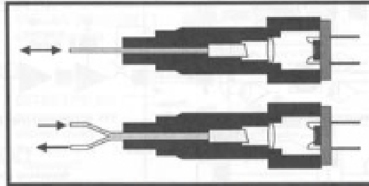
One and two fiber coaxial packages
